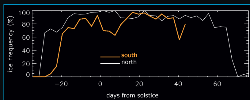
SOFIE Northern and Southern Season Ice Measurement Frequency
