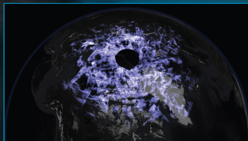
SOFIE Northern and Southern Season Ice Measurement Frequency
