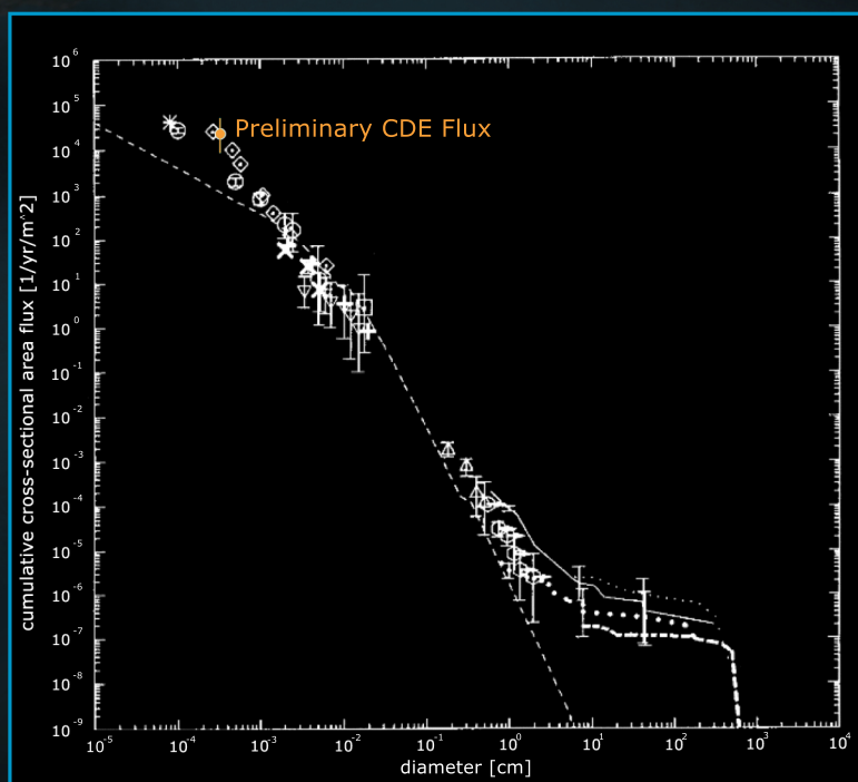
CDE Observations In Agreement with Previous Estimates of Dust Influx
